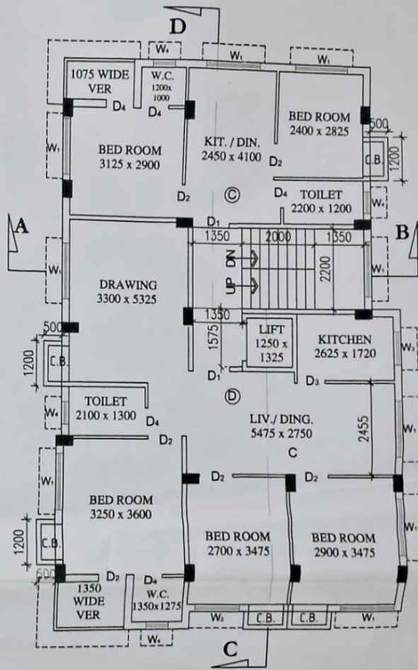
THIRD FLOOR PLAN SCALE : 1:100
